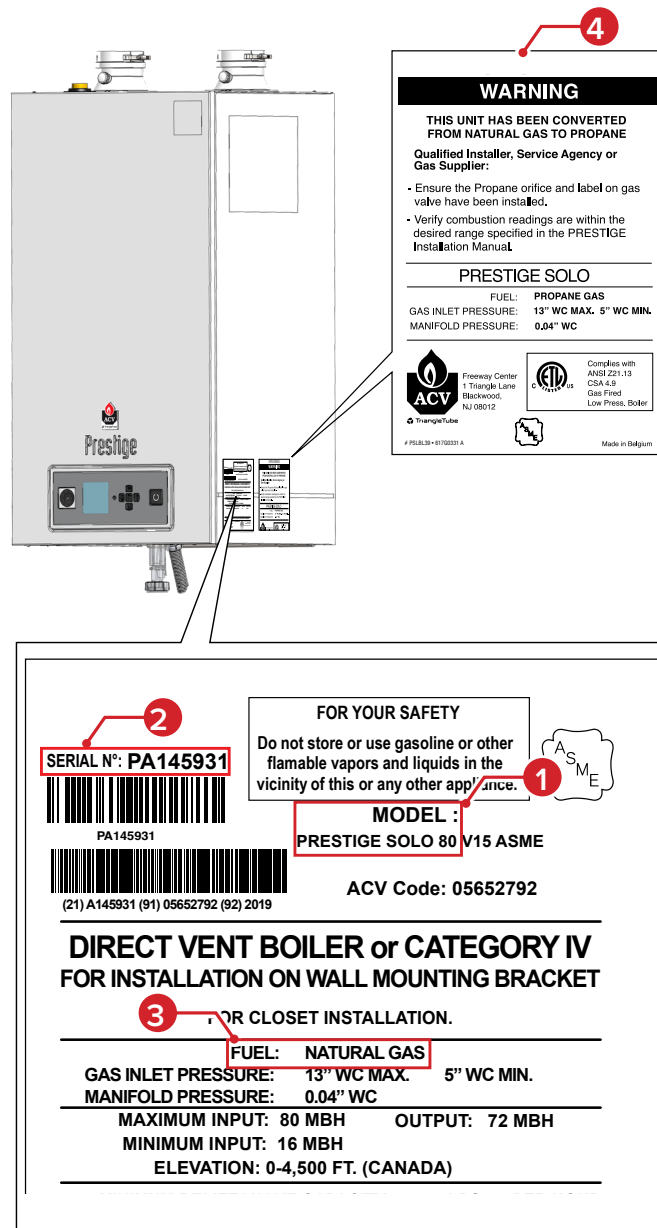
Fig. 2 - Location of Rating Label and Details on PA Boilers
