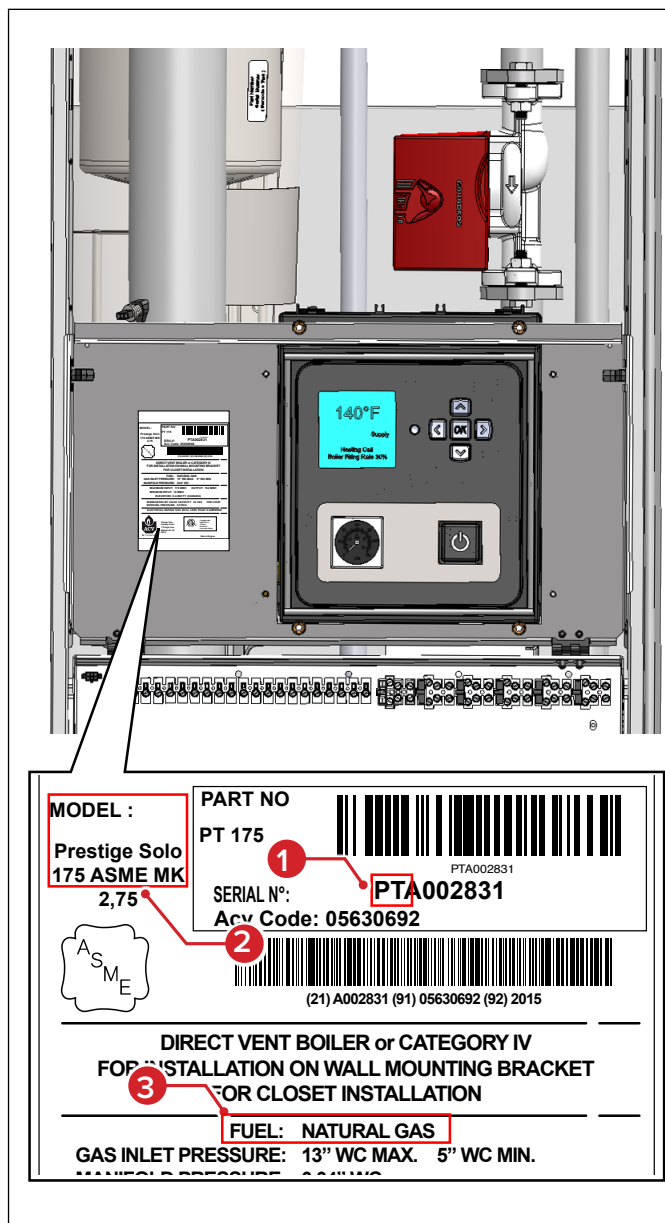
Fig. 1- Location of Rating Label and Details on PT Boilers
